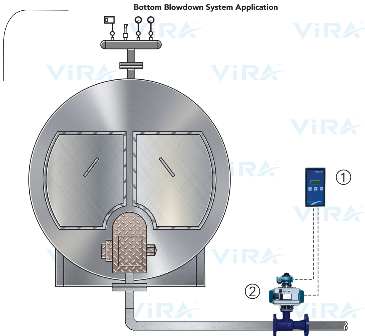
1- BK 4000 Automatic Bottom Blowdown Controller 2- BKV 4000 Automatic Bottom Blowdown Valve
